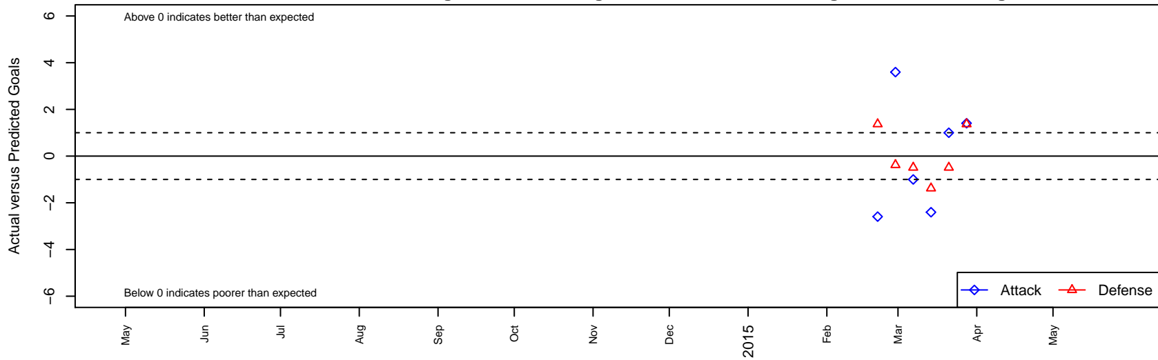
Crossfire Select Mix B02 Dots are actual minus expected GF (blue circles) and GA (red triangles). Blue line is smoothed change in attack strength. Red is smoothed change in defense strength.
